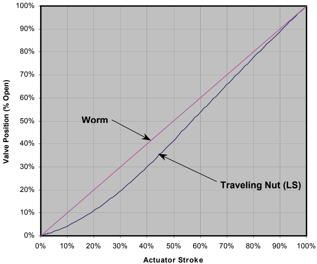
Traveling Nut vs. Worm Gear
