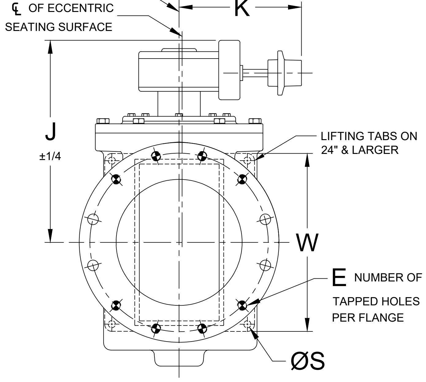
DIMENSIONS, INCHES
