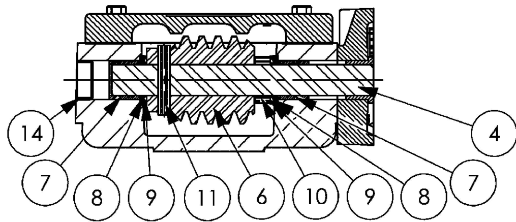
SECTION B-B
